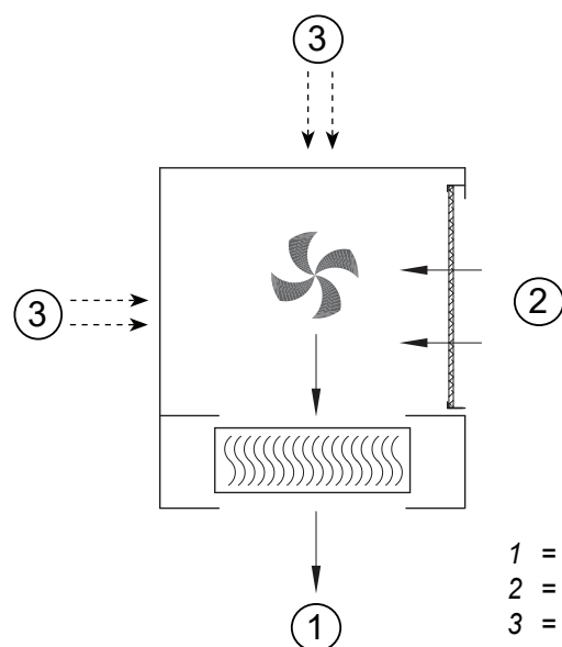
Downflow version
